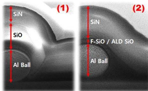
Figure 2. Cross-sectional views of two kinds of TFEs in particle environments. The particle is coated by general SiO (figure 2-1) and flowable SiO (figure 2-2).
