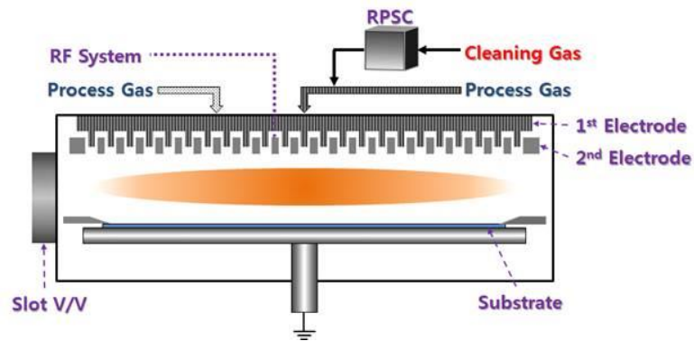
Figure 1. Schematic diagram of the TSD ALD CVD hybrid system.
