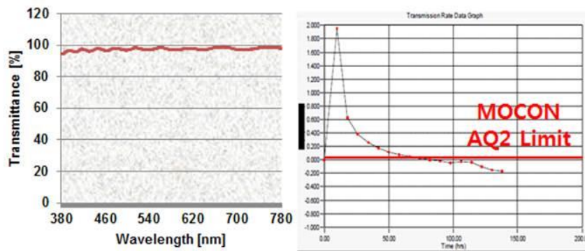
Figure 3. Characteristics of the JUSUNG TFE in particle environments.
