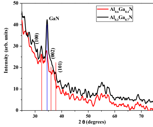
Fig. 1 XRD spectra of \text{Al}_{0.3}\text{Ga}_{0.7}\text{N} and \text{Al}_{0.6}\text{Ga}_{0.4}\text{N} thin films.
