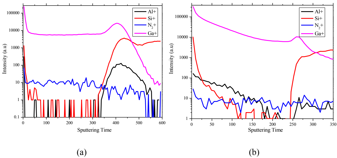
Fig. 3 SIMS profile distribution of \text{Al}_{0.3}\text{Ga}_{0.7}\text{N} (a) and \text{Al}_{0.6}\text{Ga}_{0.4}\text{N} (b)
