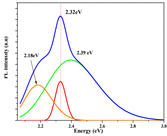
Fig. 2 Photoluminescence of \text{Al}_{0.3}\text{Ga}_{0.7}\text{N}
