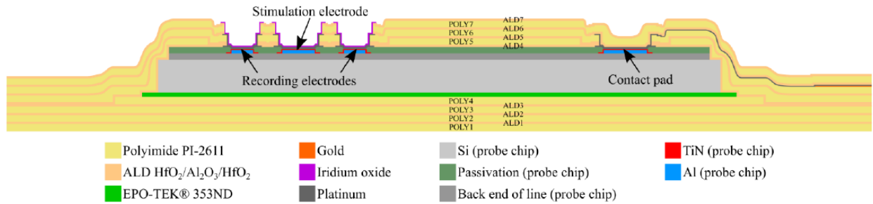
Figure 2: Schematic cross section of the encapsulated probe chip.[1]
