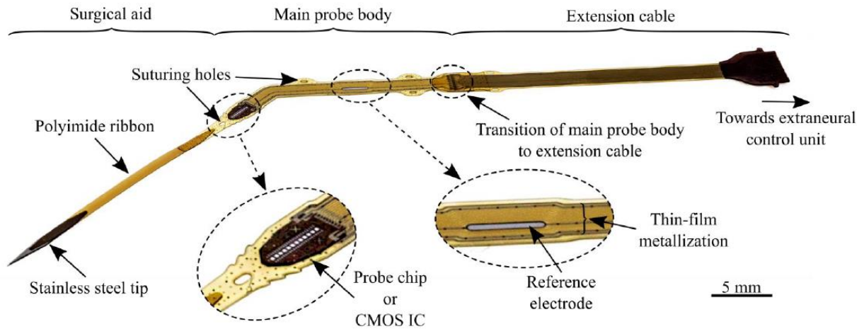
Figure 1: Overview of the hd TIME probe: indication of the different parts.[1]
