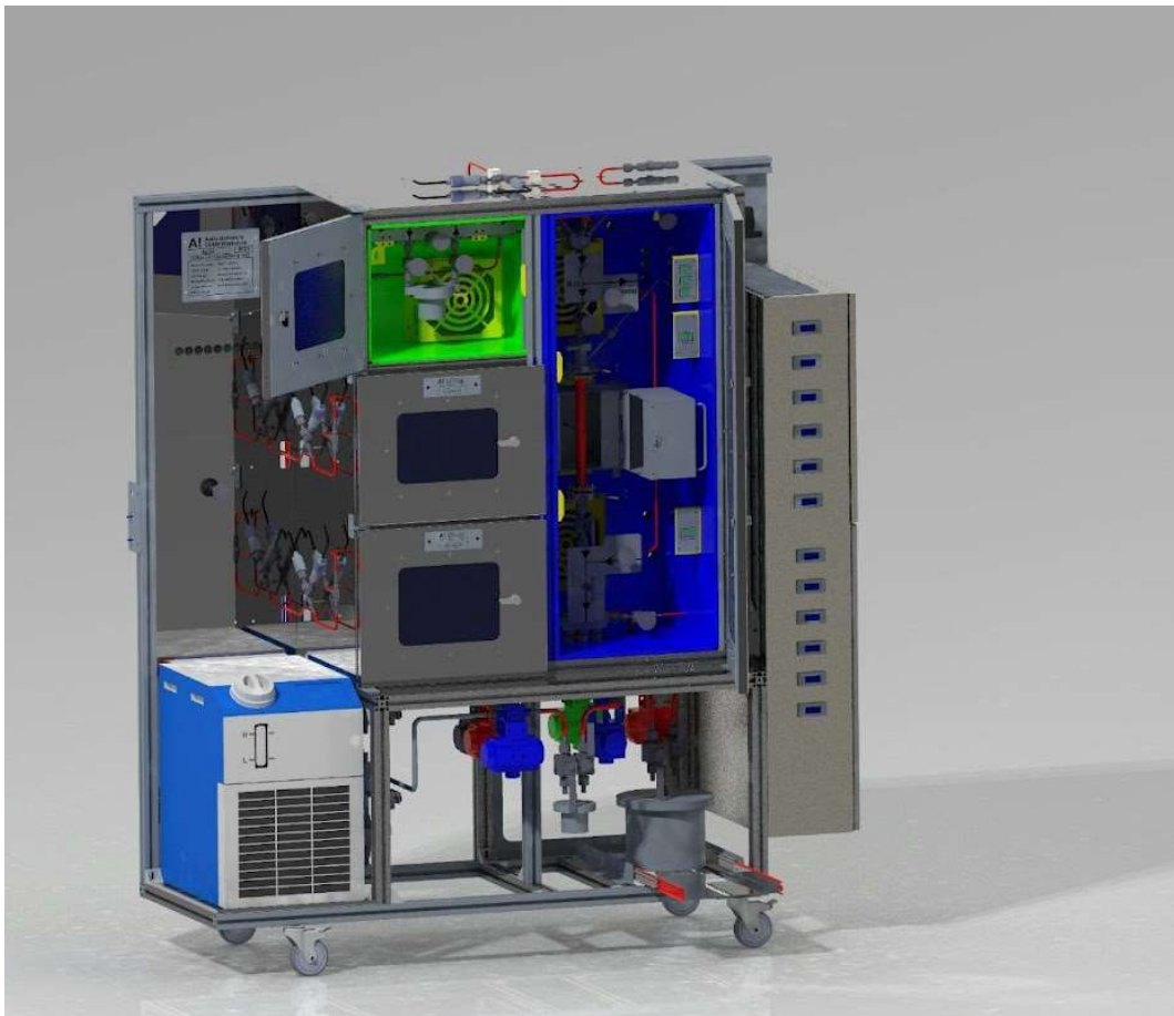
Figure 1. 3D model of the new particle ALD reactor.
