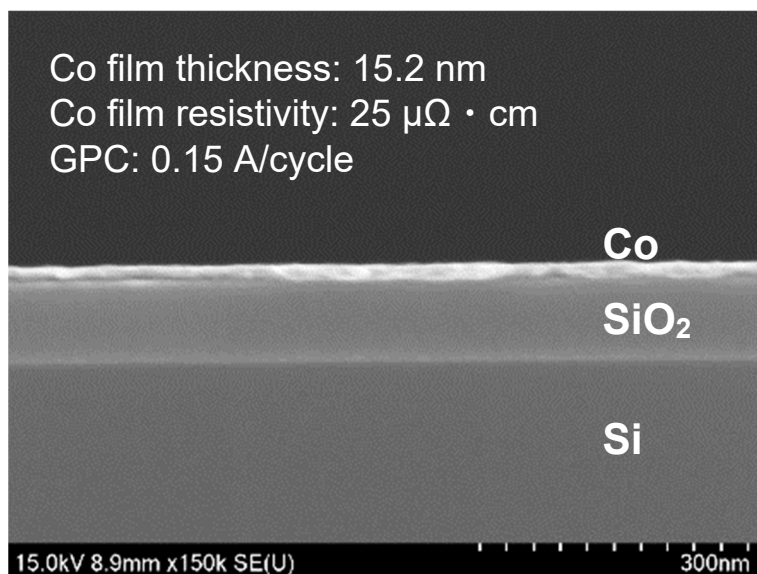
Fig.3: PEALD Co film grown with SCBA-1 (150°C) followed by PDA (350°C)
