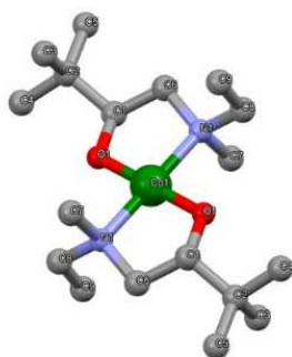
Fig.2: X-ray single crystal structure of SCBA-1
