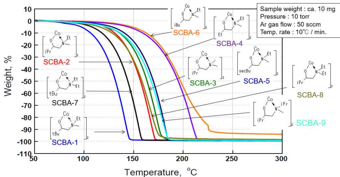
Fig.1: TGA spectra of Co-aminoalkoxides (under 10torr)
