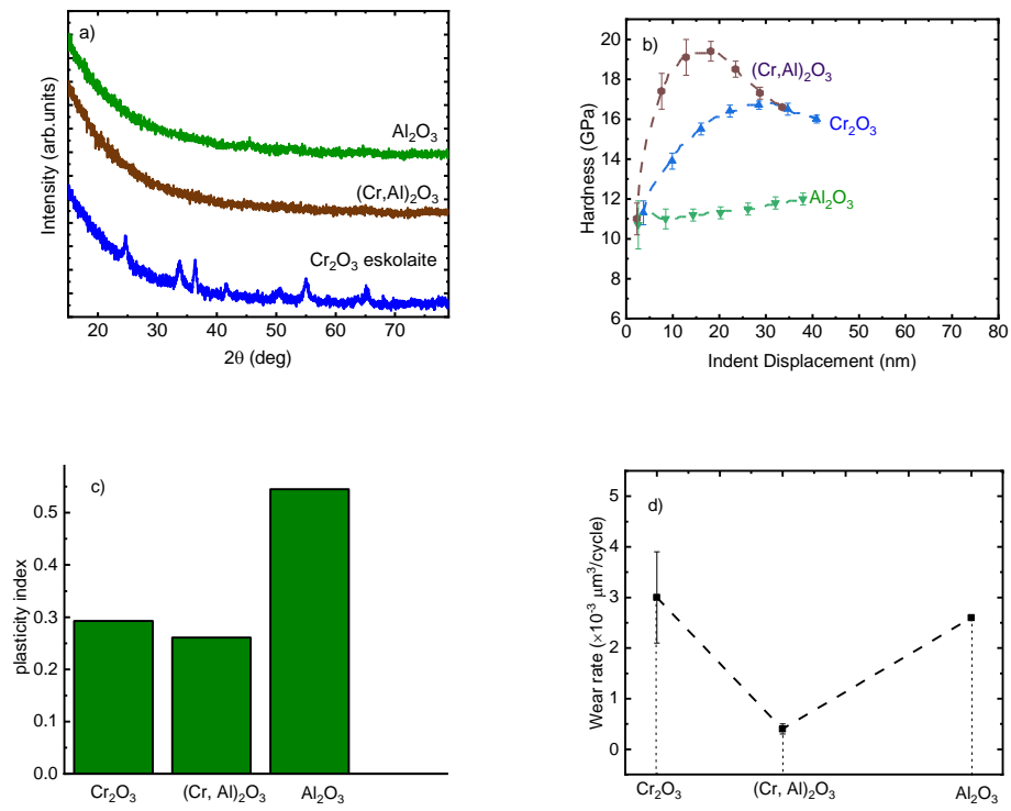
Fig. 1 Comparison of a) GIXRD patterns, b) hardness, c) plasticity index and d) wear rate of ternary (\text{Cr, Al})_2\text{O}_3 and binary \text{Cr}_2\text{O}_3 , \text{Al}_2\text{O}_3 films.
