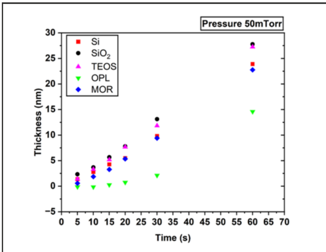
Figure 1: Ellipsometry Measurements showing Time Splits of (ASD) by (PECVD)
