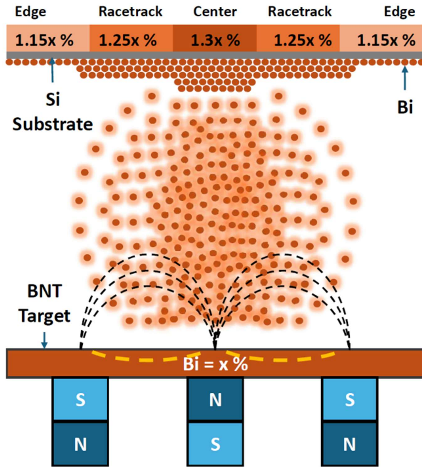
Figure 1: Illustrating the ballistic transport of Bi that causes its excess deposition compared to the lighter elements inside the growing films.
