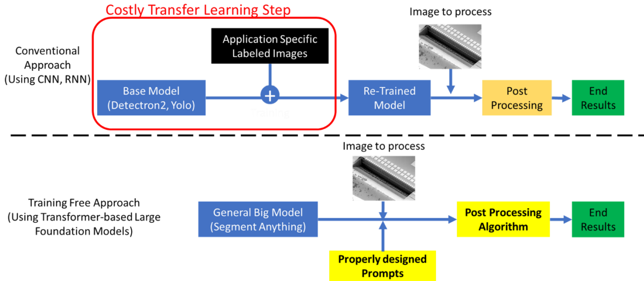
Figure 1: Workflow Comparison Between Conventional Approach vs Training free Approach
