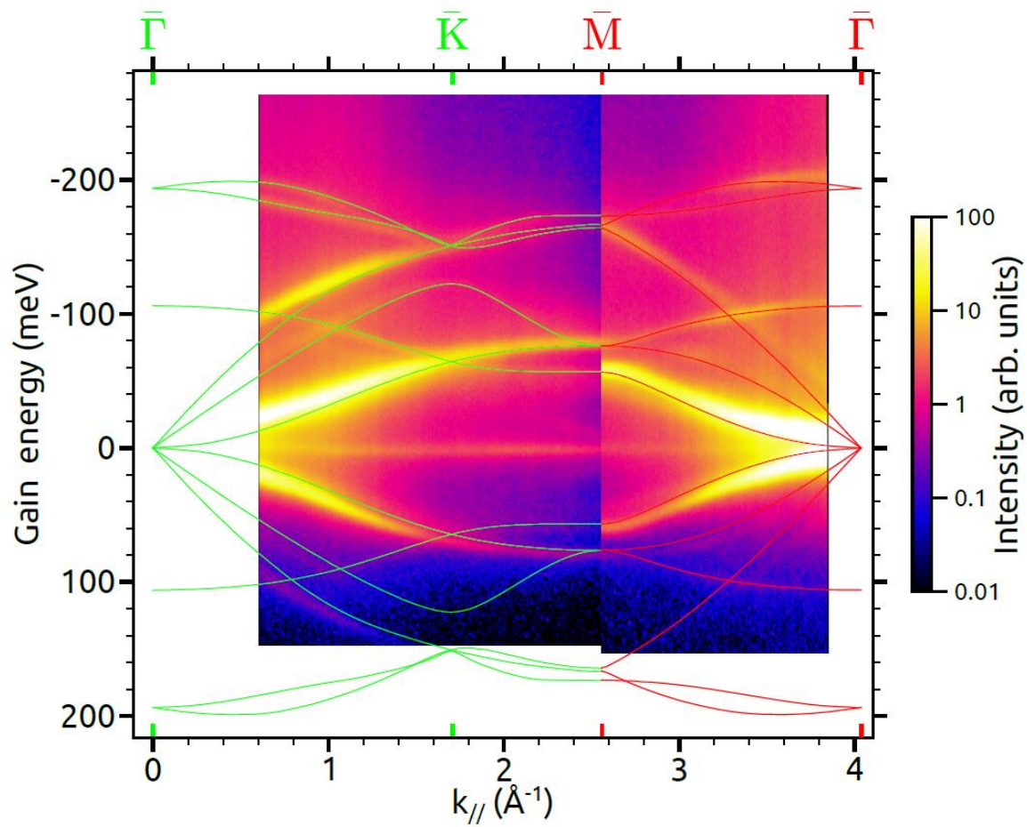
Figure 1. Phonon dispersion of single crystal graphite measured using multichannel HREELS.
