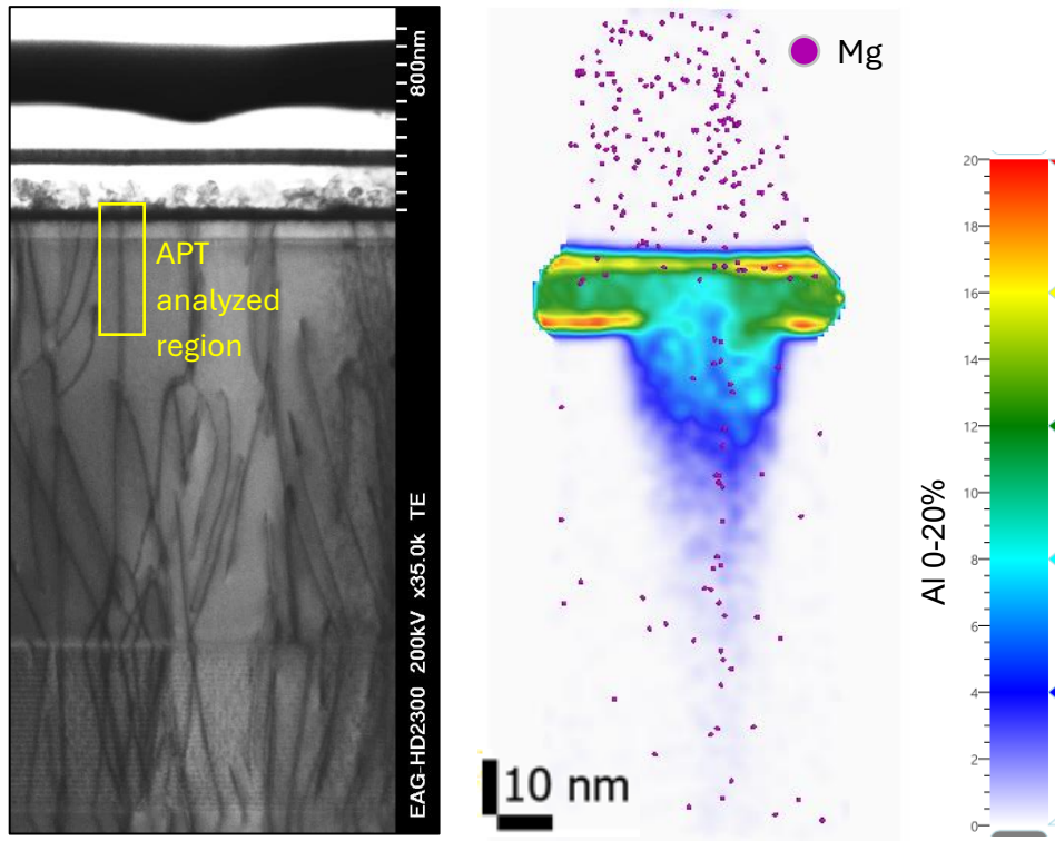
Figure. STEM image of a GaN device exhibiting a high threading dislocation density. The highlighted dislocation containing region was subsequently analyzed using APT. The 2D contour map obtained using APT, illustrating Al concentration ranging between 0-20 at.% overlaid with Mg distribution represented by purple dots. The diffusion of Mg along a linear feature into the bottom GaN is evident.
