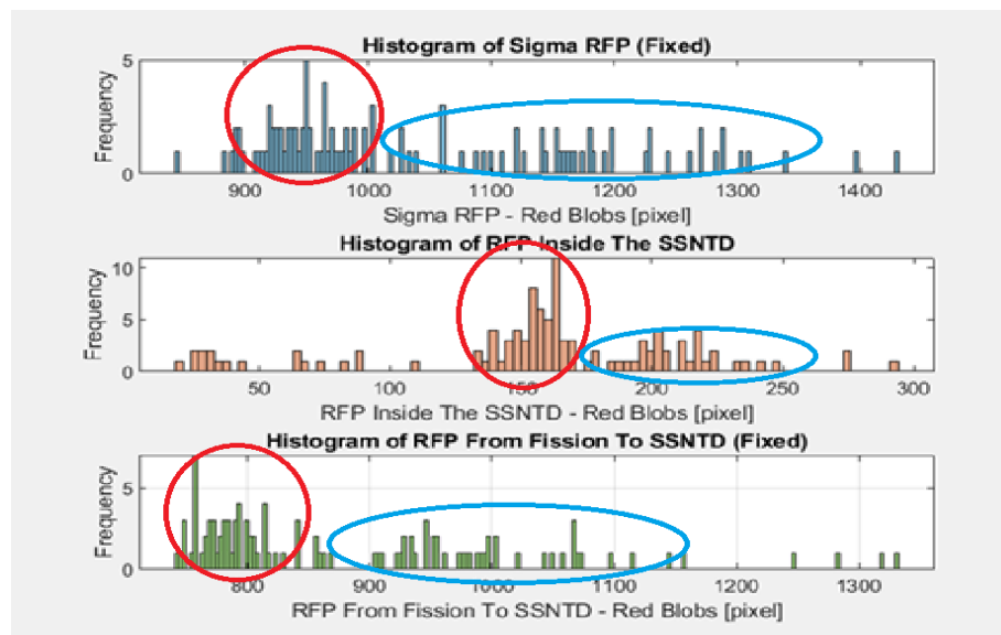
Fig 3. Fission track analysis of ^{235}\text{U} star. Lower fission track length before the detector. Middle fission track length in the detector. Upper fission track length from fission to the detector.
