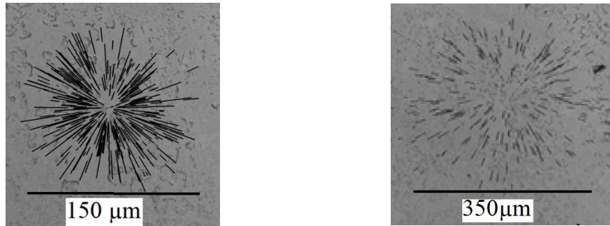
Fig 1. Fission track picture without aerogel (Left), Fission track length analysis with 4μm aerogel (Right).
