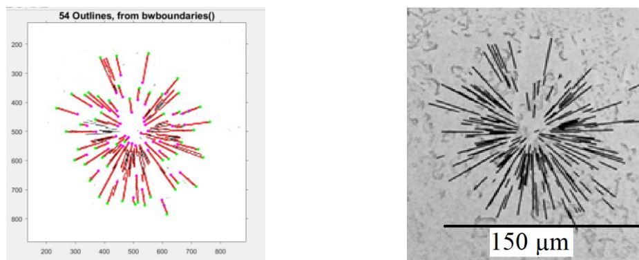
Fig 2. Fission track image (Left), Fission track length analysis (Right).
