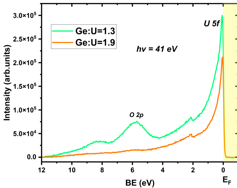
Figure 1: UPS valence band spectra of U-Ge films acquired using UPS with the He II excitation line.
