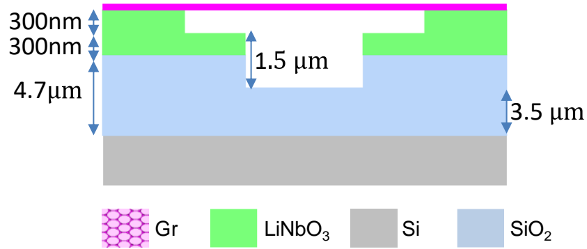
Figure: 2D schematic of the suspended multilayer graphene membrane over a dual-depth trench on a lithium niobate-on-insulator (LNOI) substrate. Material color key: Multilayer graphene (magenta), lithium niobate (green), silicon dioxide (blue), silicon substrate (gray).
