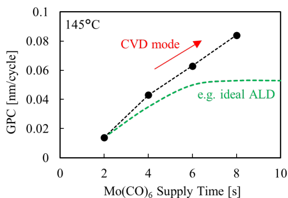
Fig.2. Dependence of GPC for \text{Mo}(\text{CO})_6 supply time.
