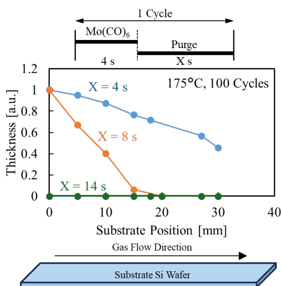
Fig.3. Film thickness at substrate position as a function of purge time
