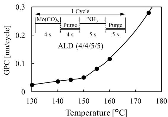
Fig.1. Dependence of GPC for ALD temperature.
