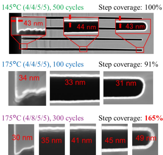
Fig.5. Step coverage in trench pattern with A/R=40 .
