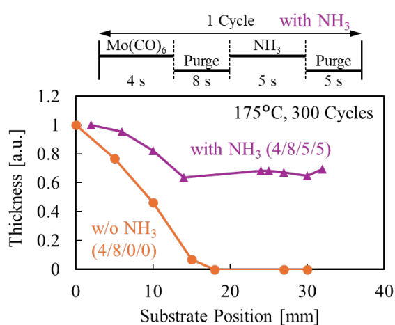
Fig.4. Film thickness at substrate position with and without \text{NH}_3 .
