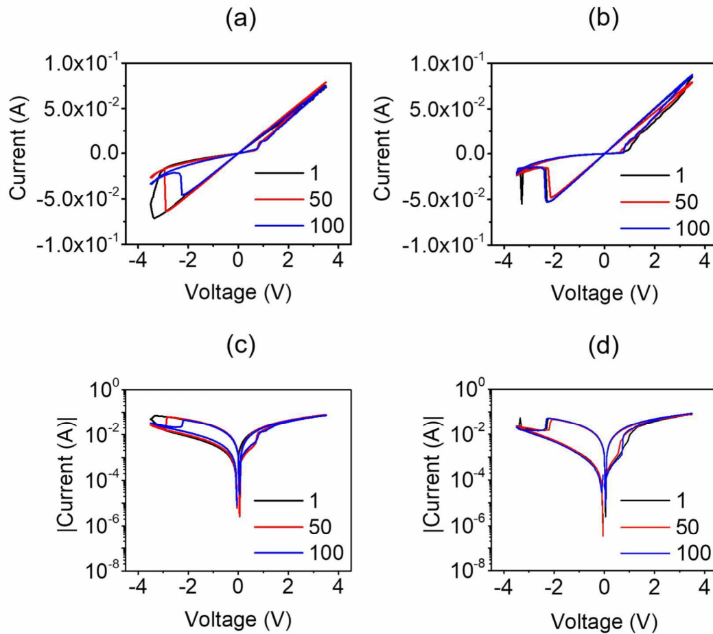
Fig. 1. 100 cycles I-V curves at (a) 40 W, (b) 80 W and log scale I-V curves of (c) 40 W and (d) 80 W after thermally assisted oxygen plasma process
