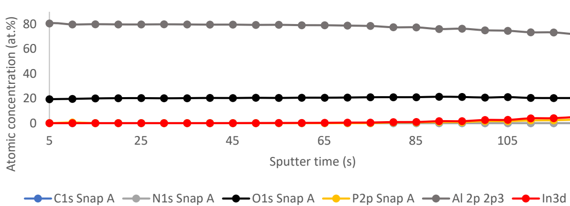
XPS Chemical Depth Profiling of the ALD N2 Sample
