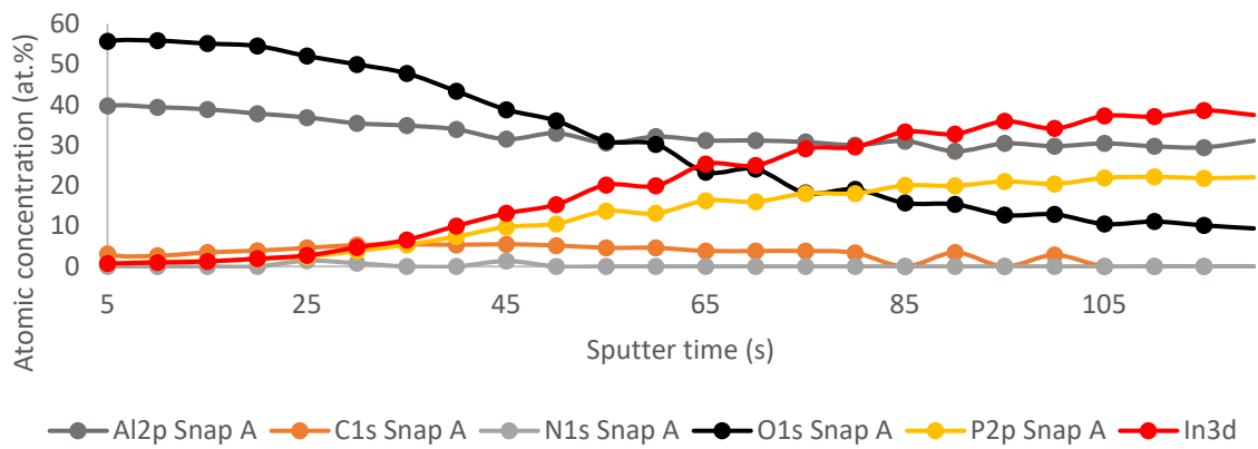
XPS Chemical Depth Profiling of the ALD Control Sample
