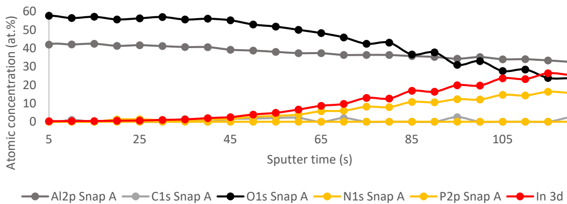
XPS Chemical Depth Profiling of the ALD O2 Sample
