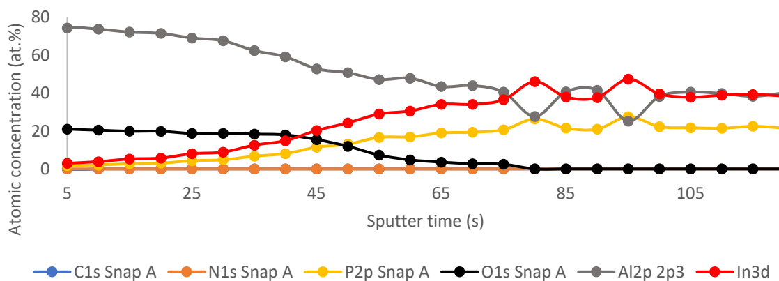
XPS Chemical Depth Profiling of the Sputtering O2 Sample
