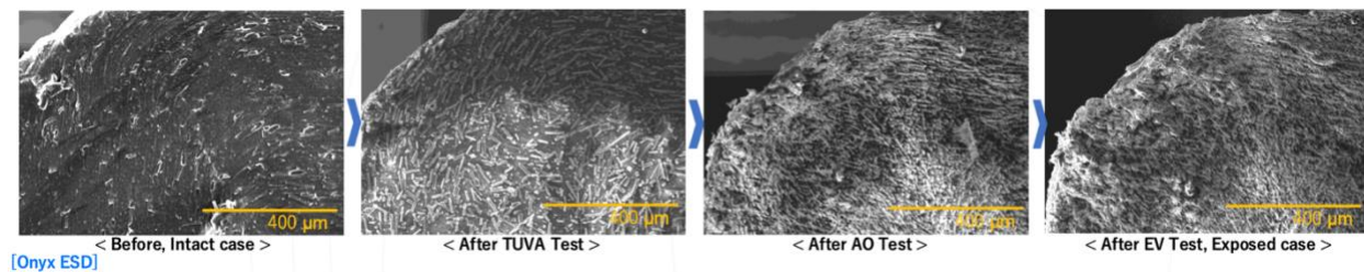
Fig 1. SEM Image (Magnification x 130) of Onyx ESD specimen corner before and after exposure to ground simulation of VLEO environment (STARLINK-11193, 2 years operation)
