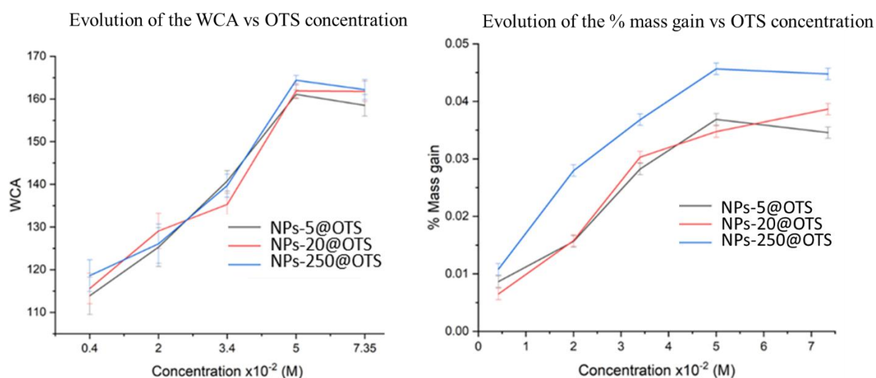
Fig. 1: Static water contact angle (left) and mass gain (right) of glass coated with OTS-functionalized silica nanoparticles (NPs-5, NPs-20 and NPs-250) as a function of OTS concentration.
