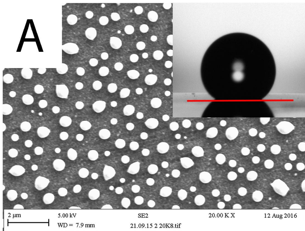
SEM images of coatings: A) PTFE-TiO 2 ; B) TiO 2 . Inserts show the water droplets on the surface of the corresponding sample
