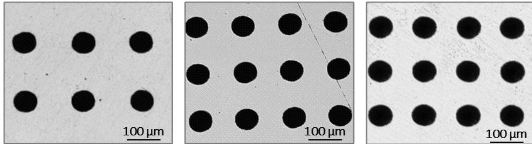
Figure 1. Confocal images of the laser-textured surfaces for micro-dimple densities of (a) 10%, (b) 15% and (c) 20%.
