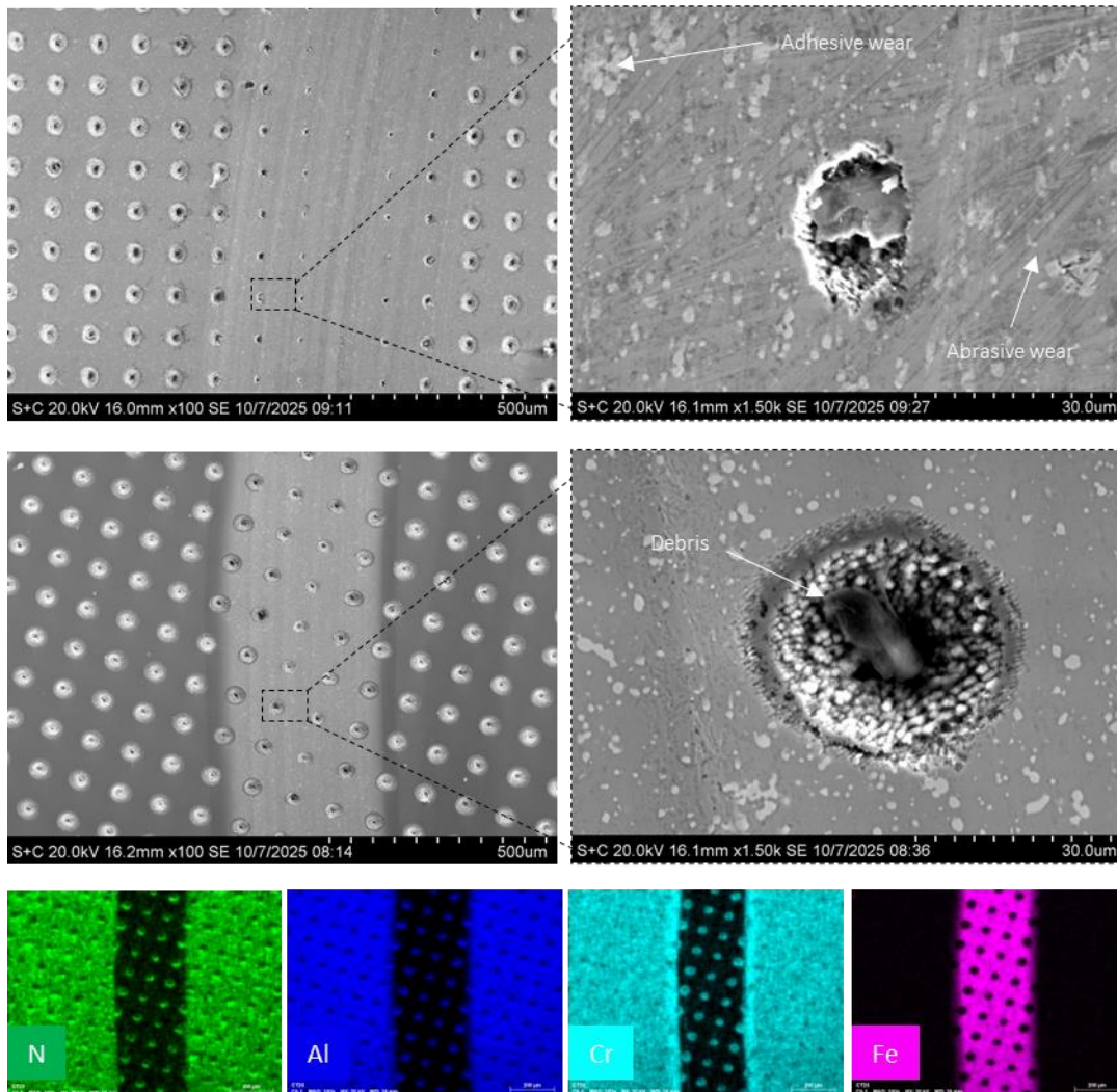
Figure 2. SEM micrographs and EDX elemental maps of the coated and uncoated worn surfaces textured with dimple densities 20% after the wear tests.
